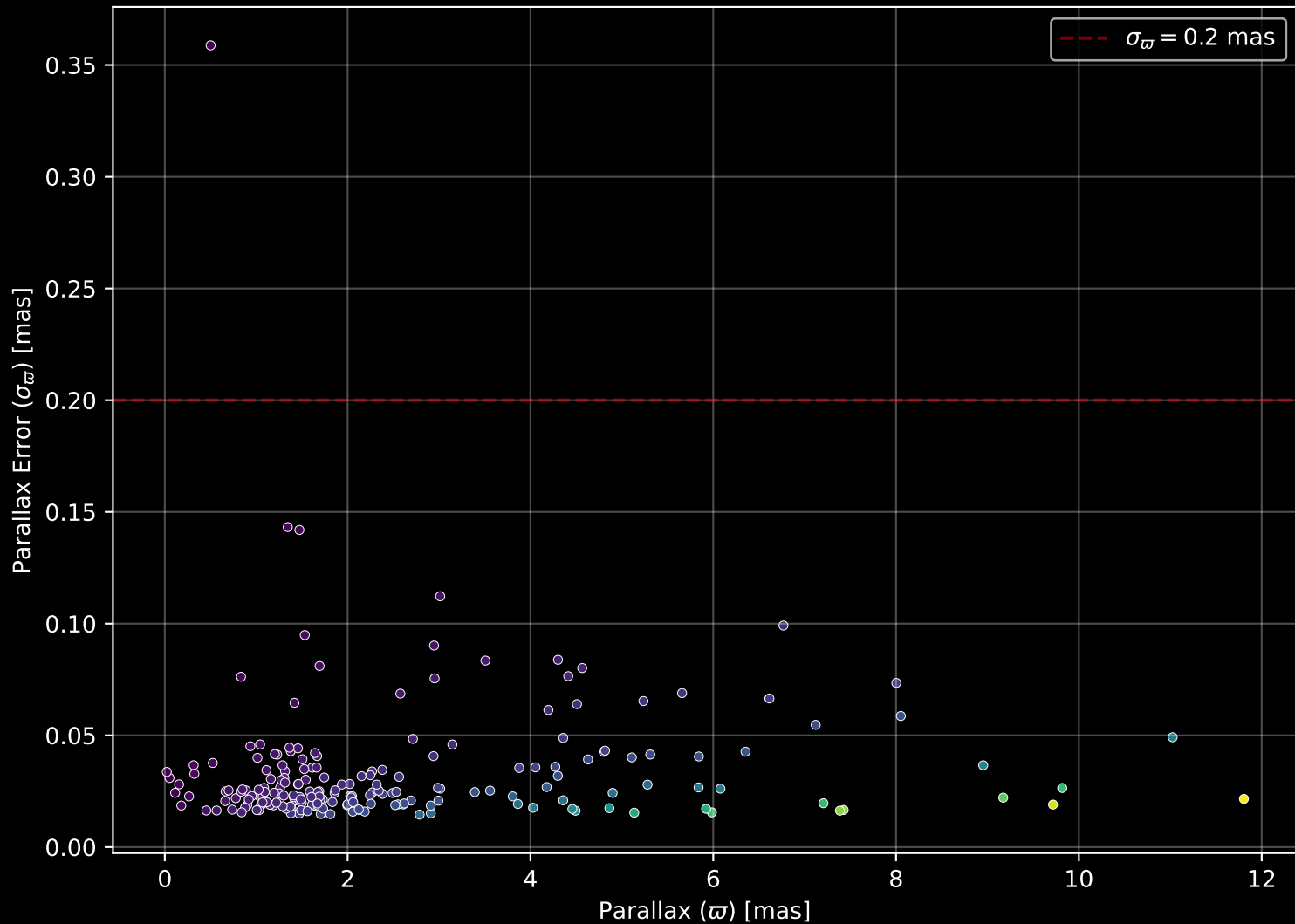
APOGEE DR17 Field: [K2_C10_285+61] Parallax Quality (n= 203)
