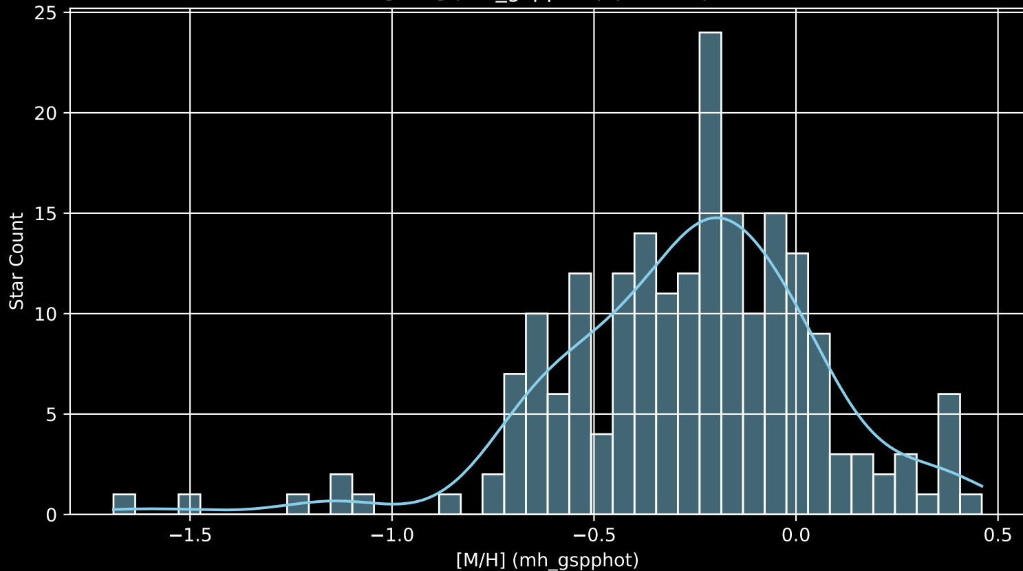
APOGEE DR17 Field: [K2_C10_285+61 [M/H] (mh_gspphot) (n= 202)
