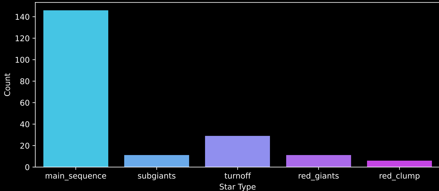
APOGEE DR17 Field: [K2_C10_285+61] Count plot of Star Type
