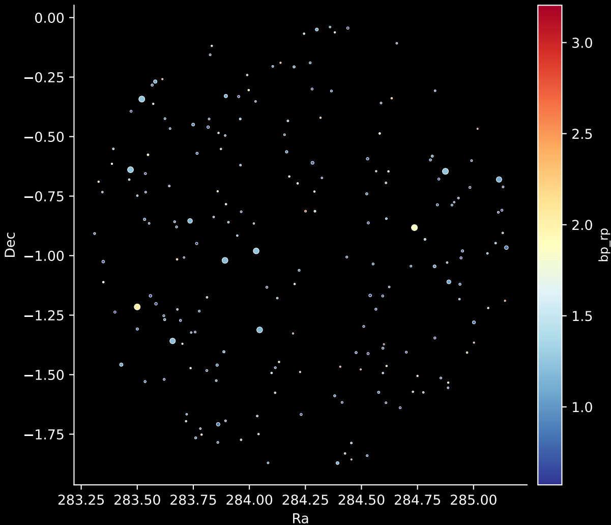
APOGEE DR17 Field: [K2_C10_285+61] Stars: 203
