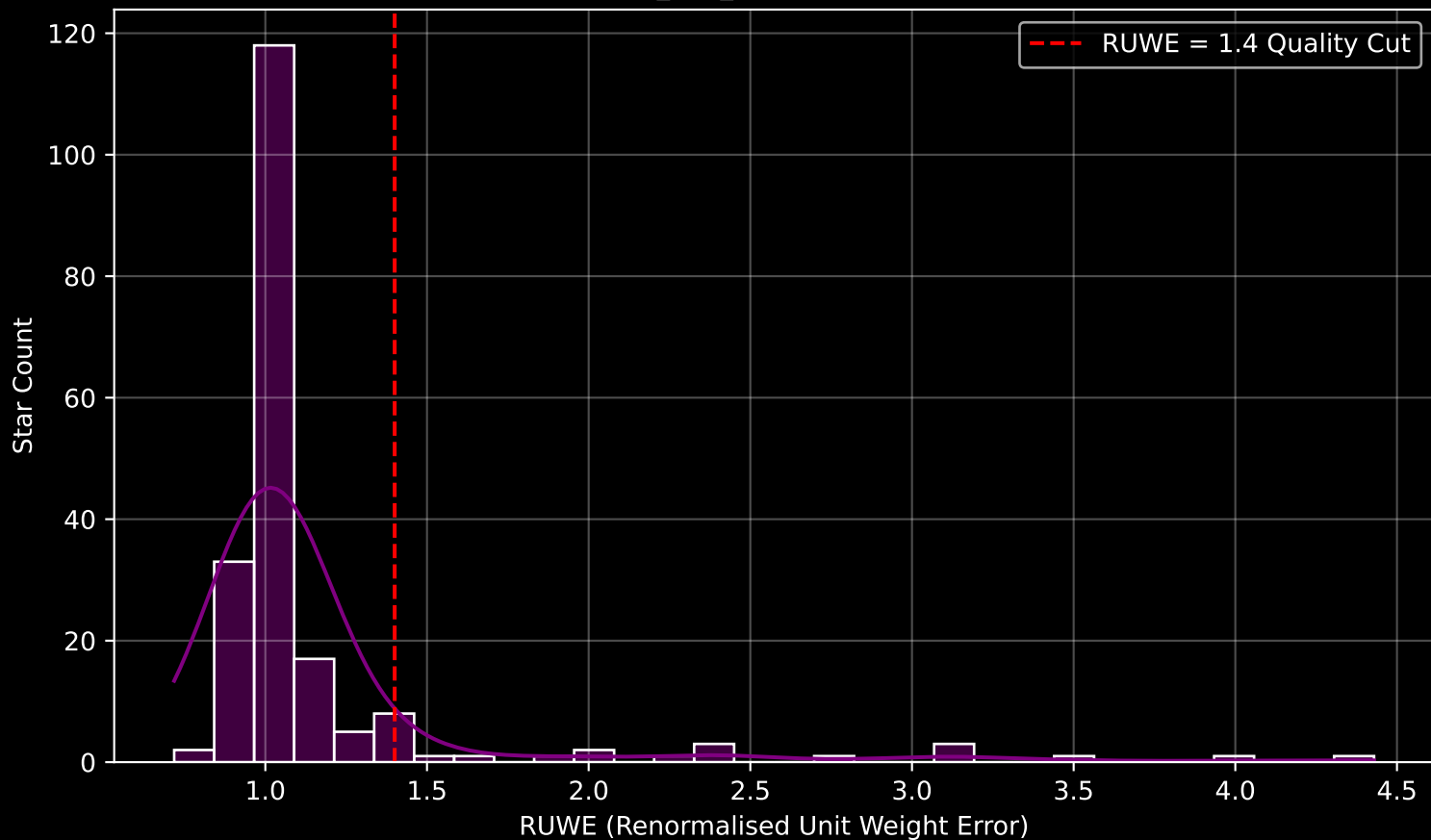
GAPOGEE DR17 Field [K2_C10_285+61] RUWE Distribution (n= 199)
