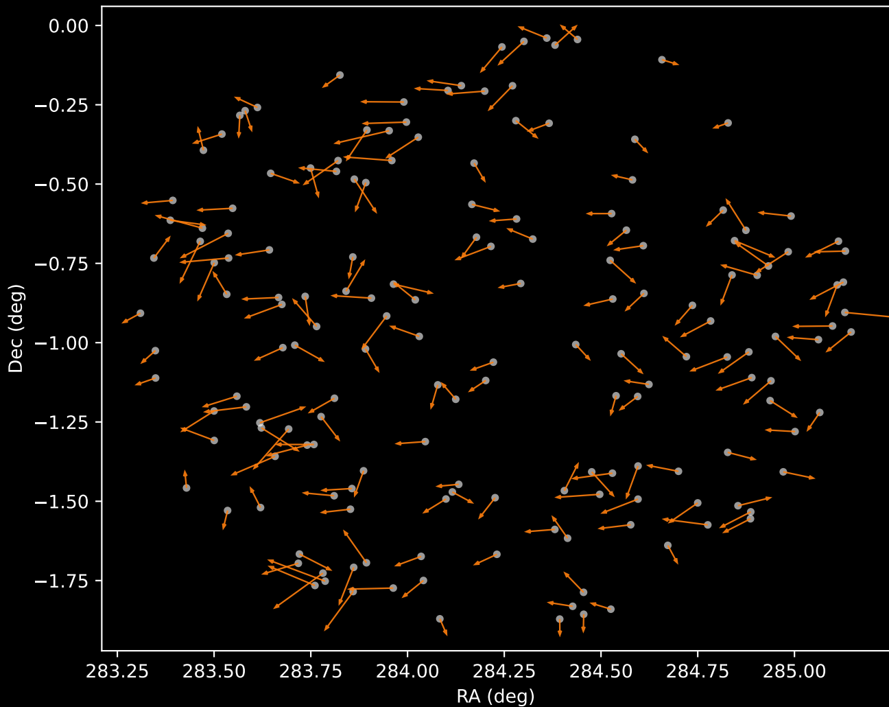
APOGEE DR17 Cluster 2 Proper Motion Vectors (n=170)
