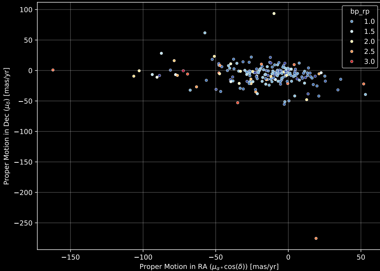
APOGEE DR17 Field: [K2_C10_285+61] Proper Motion Diagram (n= 203)
