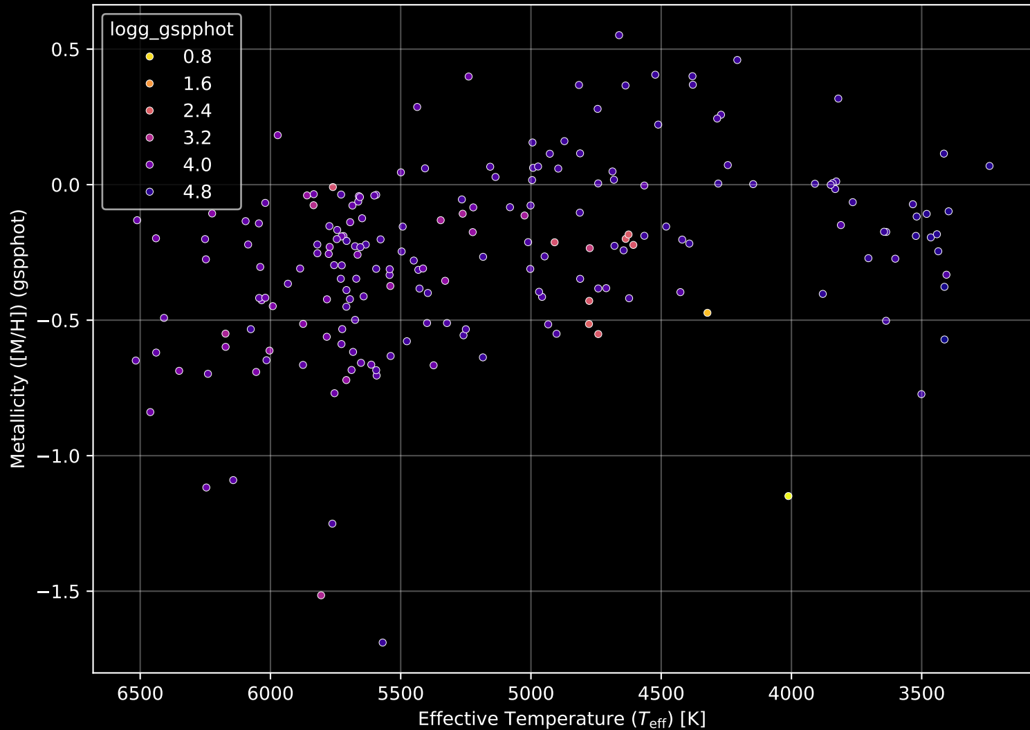
APOGEE DR17 Field: [K2_C10_285+61] Stellar Population Parameters (n= 203)
